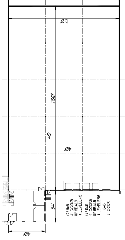
FLOOR PLAN
